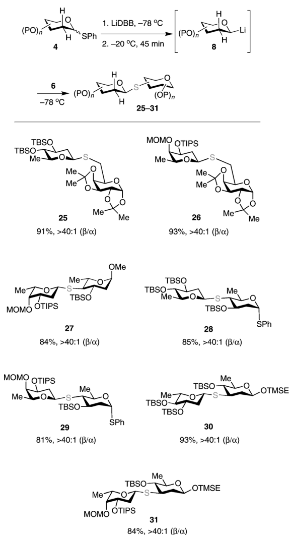
Scheme 4. Synthesis of S-linked 2-deoxy- \beta -glycosides. General conditions: 2-deoxyglycosyl phenylsulfide (2.0 equiv), LiDBB (4.4 equiv), -78^{\circ}\text{C} , 15 min; then left to stand at -20^{\circ}\text{C} for 45 min; disulfide acceptor (1.0 equiv), THF, -78^{\circ}\text{C} , 5 h. In each case, the yield of the S-linked 2-deoxy- \beta -glycoside is given.
