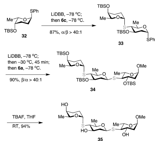
Scheme 5. Stereoselective synthesis of an S-linked 2-deoxytrisaccharide.
